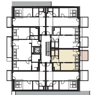
1.DG STRASSESTRAKT
